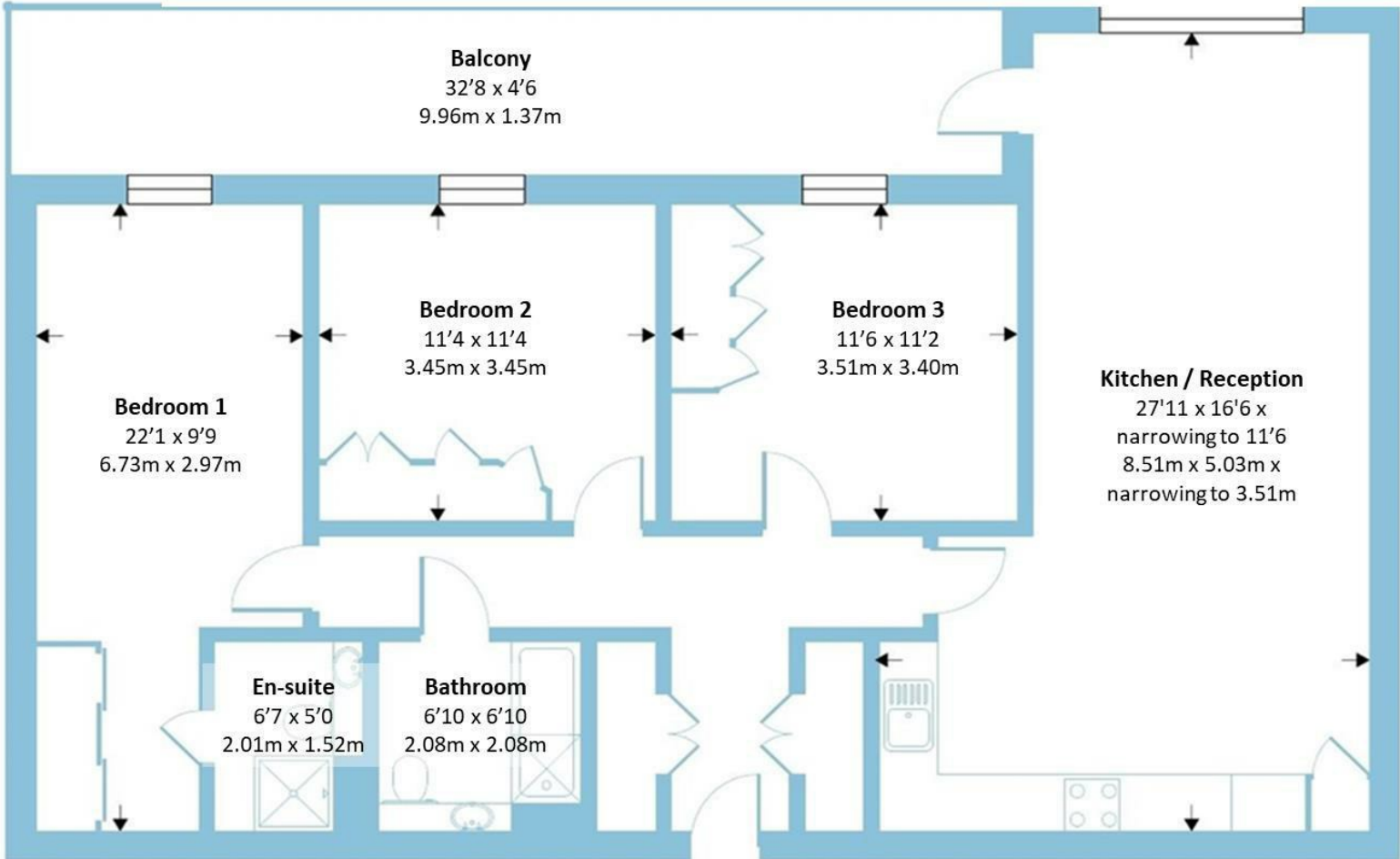
FIRST FLOOR
